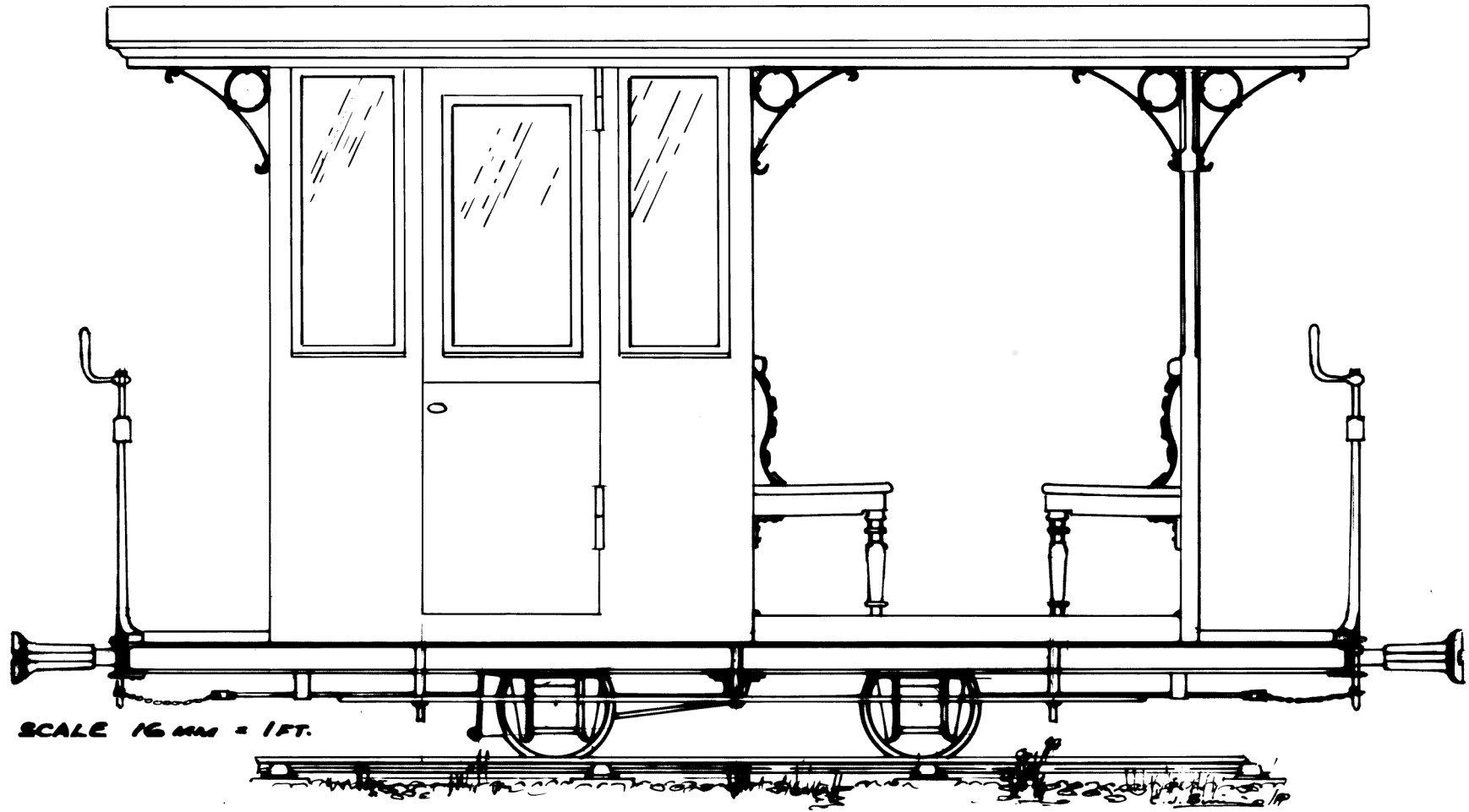
→ FOUR WHEELED COACH BY ARTHUR KOPPEL SOURCE - KOPPEL CATALOGUE ILLUSTRATION
