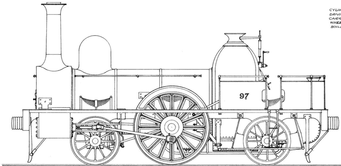
L.B. & S.C.R. 2-2-2 TANK ENGINE NO 97 BUILT BY MESSRS. JONES & POTTS & REBUILT AT BRIGHTON 1852.
