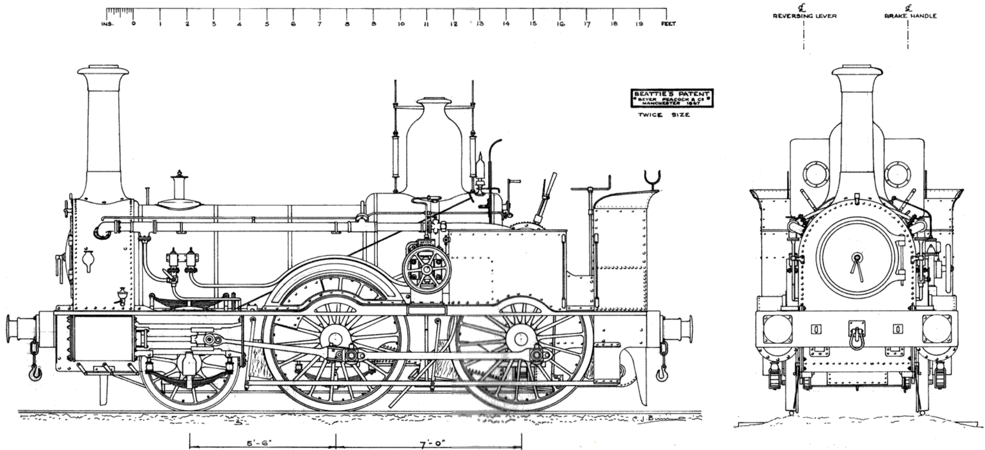
L.S.W.R. 2-4-0 WT. - DESIGNED BY J. BEATTIE - AS BUILT 1867 BY BEYER-PEACOCK. (Nos 243 to 254 incl.)
